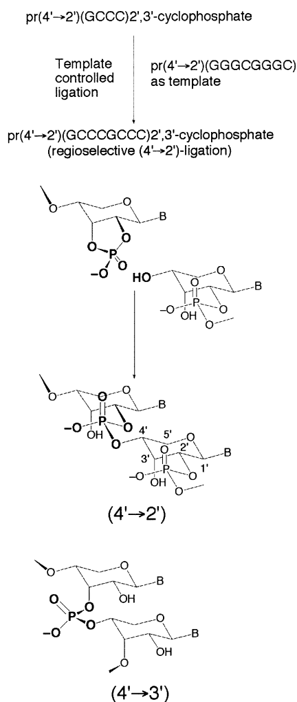
Scheme 3. Template-controlled ligation of (4'→2')-(D)-β-ribo-pyranosyl tetramer cyclophosphates leading to regioselective (4'→2') as against their 4'→3')-ligation product (from ref 15).
