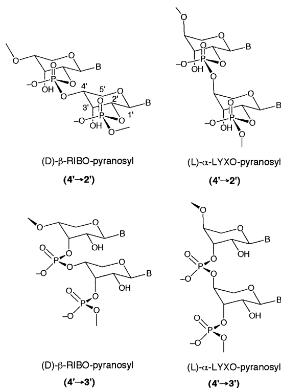
Scheme 2. (4'→2')-(D)-β-ribo- and (4'→2')-(L)-α-lyxo-pyranosyl oligonucleotides and their corresponding (4'→3')-pentopyranosyl counterparts in their idealized pairing conformations.
