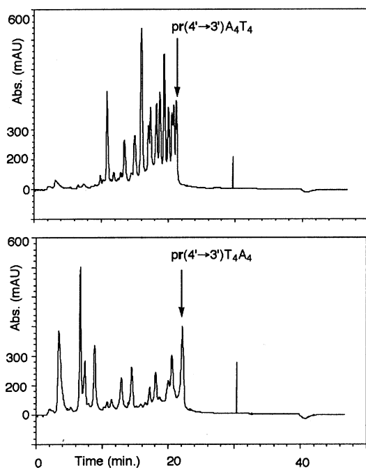
Figure 5. HPLC trace of the crude, fully deprotected, (D)- \beta -ribofuranosyl(4'→3')-oligonucleotides, pr(4'→3')(A 4 T 4 ) and pr(4'→3')(T 4 A 4 ). For conditions of chromatography, see Table 1.
