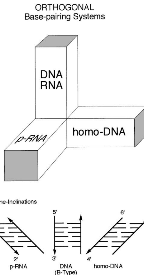
Figure 3. The three groups of base-pairing systems which exhibit strong intrasystem base-pairing but do not cross communicate with each other; they represent orthogonal base-pairing systems. This orthogonality is proposed to be related to the different backbone/basepair-axes inclinations of these systems.
