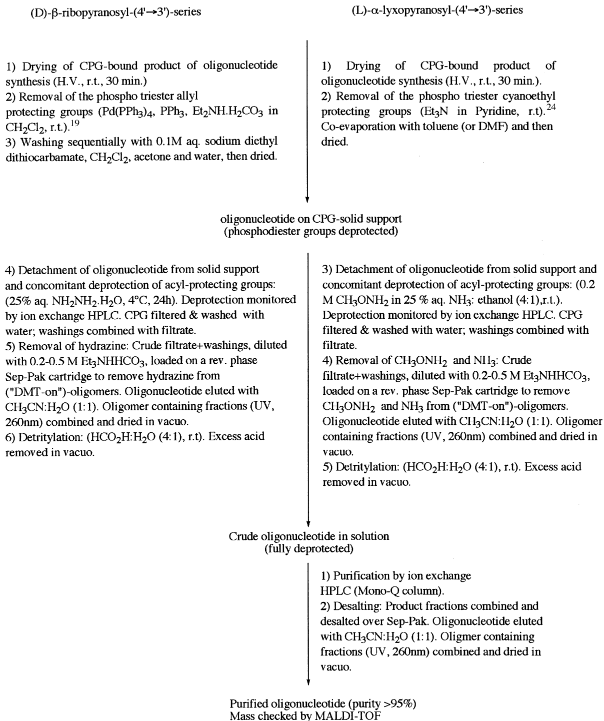
Scheme 6. The deprotection, purification and isolation protocols followed in the (4'→3')-(D)- \beta -ribo- and (4'→3')-(L)- \alpha -lyxo-pyranosyl oligonucleotide series.
