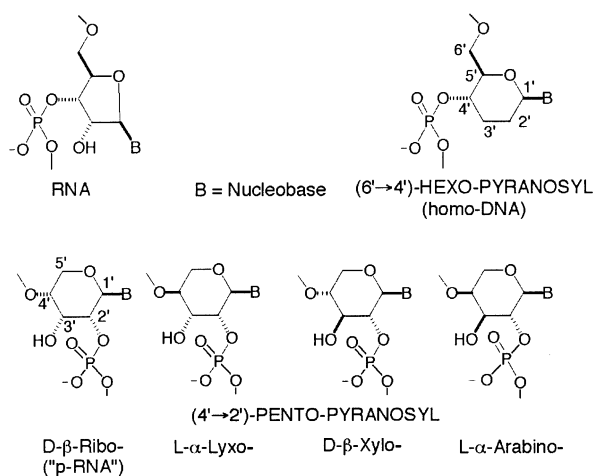
Scheme 1. Constitution and configuration of the repeating units of RNA, homo-DNA, and the family of the four (4'→2')-pentopyranosyl oligonucleotides.
