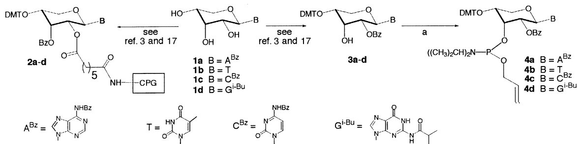
Scheme 4. Preparation of the A, T, G and C building blocks in the (4'→3')-(D)-β-ribo-pyranosyl series. 3a(3b, 3c, 3d)→4a (4b, 4c, 4d): (a) (allyloxy)(diisopropylamino)chlorophosphine, diisopropyl ethyl amine, CH 2 Cl 2 , rt, 94% (78%, 63%, 63%). DMT = 4,4'-dimethoxy trityl. CPG = long-chain-alkylamino-controlled pore glass.
