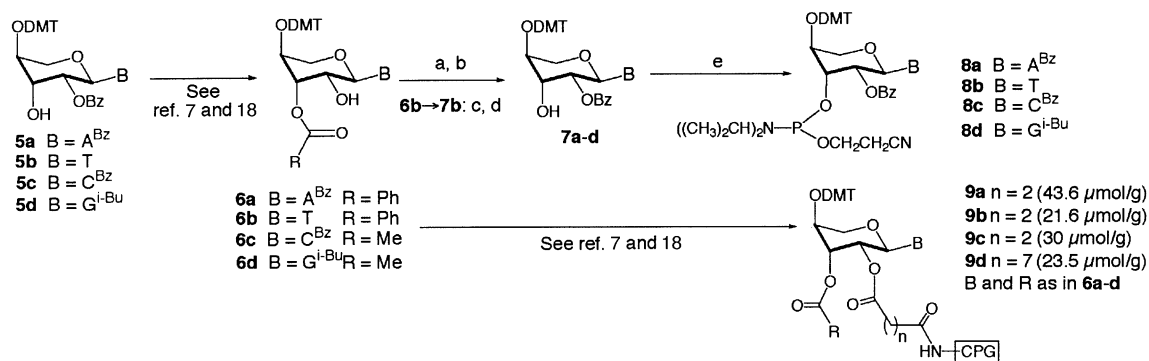
Scheme 5. Preparation of the A, T, G and C building blocks in the (4'→3')-(L)- \alpha -lyxopyranosyl series. 6a ( 6c , 6d )→ 7a ( 7c , 7d ): (a) aq NaOH in THF, H 2 O (2:1), 0 °C; (b) benzoyl chloride, pyridine, 0 °C, 90% (87%, 95%). 6b → 7b : (c) K 2 CO 3 in MeOH, 0 °C; (d) benzoyl chloride, pyridine, 0 °C, 91%. 7a ( 7b , 7c , 7d )→ 8a ( 8b , 8c , 8d ): (e) (2-cyanoethoxy)(diisopropylamino)chlorophosphine, 2,4,6-collidine, 0.5 equiv N -methylimidazole, CH 2 Cl 2 , rt, 73% (82%, 70%, 72%). DMT = 4,4'-dimethoxy trityl; CPG = long-chain-alkylamino-controlled pore glass.
