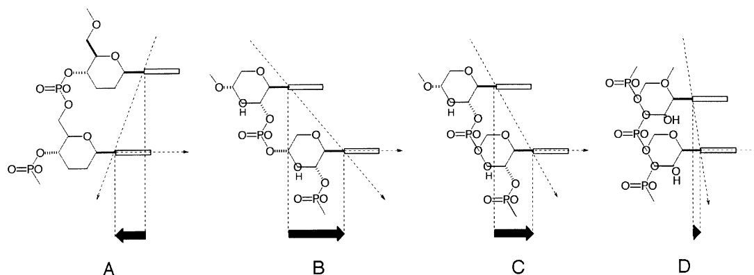
Figure 4. Qualitative vertical projections of formulas of the pairing conformations (idealized, nucleosidic torsion angles -120^\circ ) of the four oligonucleotide systems: (A) homo-DNA (g/t phosphodiester conformation); (B) pyranosyl-RNA; (C) (4' \rightarrow 2') -(L)- \alpha -lyxopyranosyl-, and D: (4' \rightarrow 3') -(L)- \alpha -lyxopyranosyl-oligonucleotides. Projections allow a rough estimate of the sense and the degree of the four systems' backbone/base-pair-axes inclination. 32 Note that sense and degree of the inclination depends sensitively on the nucleosidic torsion angle.
