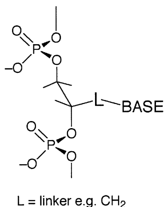
Scheme 7. A hypothetical aliphatic oligonucleotide backbone system in which the vicinal phosphodiester groups might—as a result of a tendency to minimize electrostatic repulsion—assume an anti-periplanar conformation.
