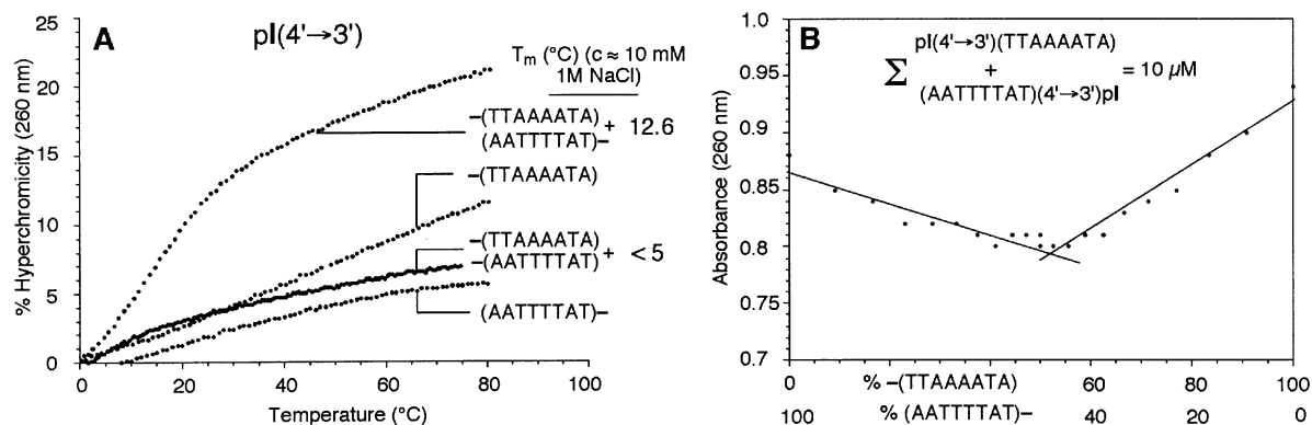
Figure 2. (A) UV- T_m curves documenting the preference of the anti-parallel pairing behavior in the (4'→3')-(L)-α-lyxoyranosyl oligonucleotide series: pl(4'→3')-(TTAAAATA) with its antiparallel complement pl(4'→3')-(TATTTTAA) strand and its parallel complement pl(4'→3')-(AATTTTAT) strand. For conditions see caption of Figure 1. (B) Molar-ratio-dependent UV spectroscopy-mixing curve indicating the 1:1 complexation stoichiometry between the sequence pl(4'→3')-(TATTTTAA) and its antiparallel complement pl(4'→3')-(TTAAAATA) (260 nm, 0 °C).
