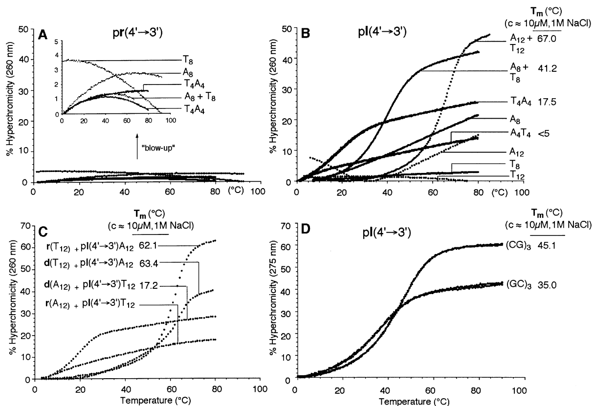
Figure 1. UV- T_m curves documenting the pairing behavior in (A) the (4'→3')-(D)-β-ribofuranosyl oligonucleotide series; curves of the non-self-complementary single strands are also shown, (B, D) (4'→3')-(L)-α-lyxoyranosyl oligonucleotide series; curves of the non-self-complementary single strands are also shown, and (C) the intersystem cross-pairing of (4'→3')-(L)-α-lyxoyranosyl oligonucleotides with RNA and DNA. All measurements were made with total oligonucleotide concentration \approx 10 \mu\text{M} in 10 mM aq \text{NaH}_2\text{PO}_4 buffer containing 0.1 mM \text{Na}_2\text{EDTA} , 150 mM \text{NaCl} at pH 7.0.
